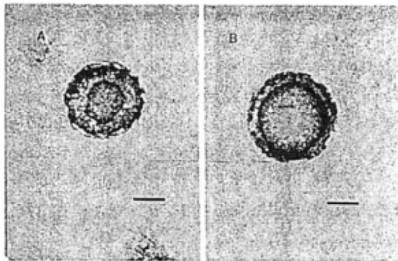
Fig. 2. Electron micrograph of isolated influenza viruses. A : influenza A/Sydney/05/97-like(H3N2), B : influenza A/Beijing/262/95-like(H1N1).
