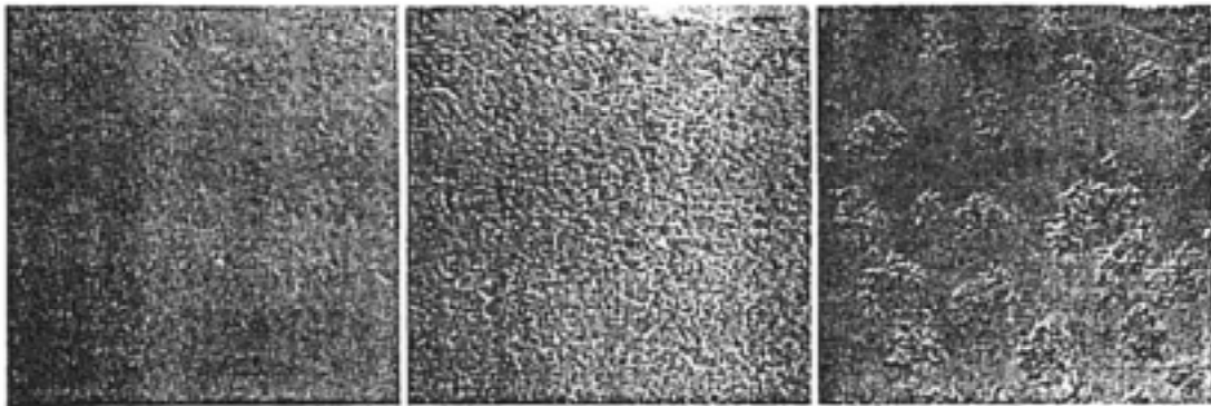
Fig. 1. Cytopathic effects on MDCK cells infected with isolated influenza virus. A : Normal cells of MDCK, B : 72-hr exposure of influenza A/Sydney/05/97-like(H3N2), C : 72-hr exposure of influenza A/Beijing/262/95-like(H1N1).
